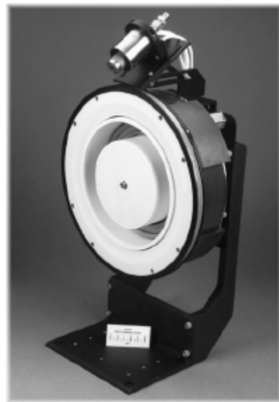
Figure 1 - Photograph of the NASA-173Mv2 Hall thruster.
